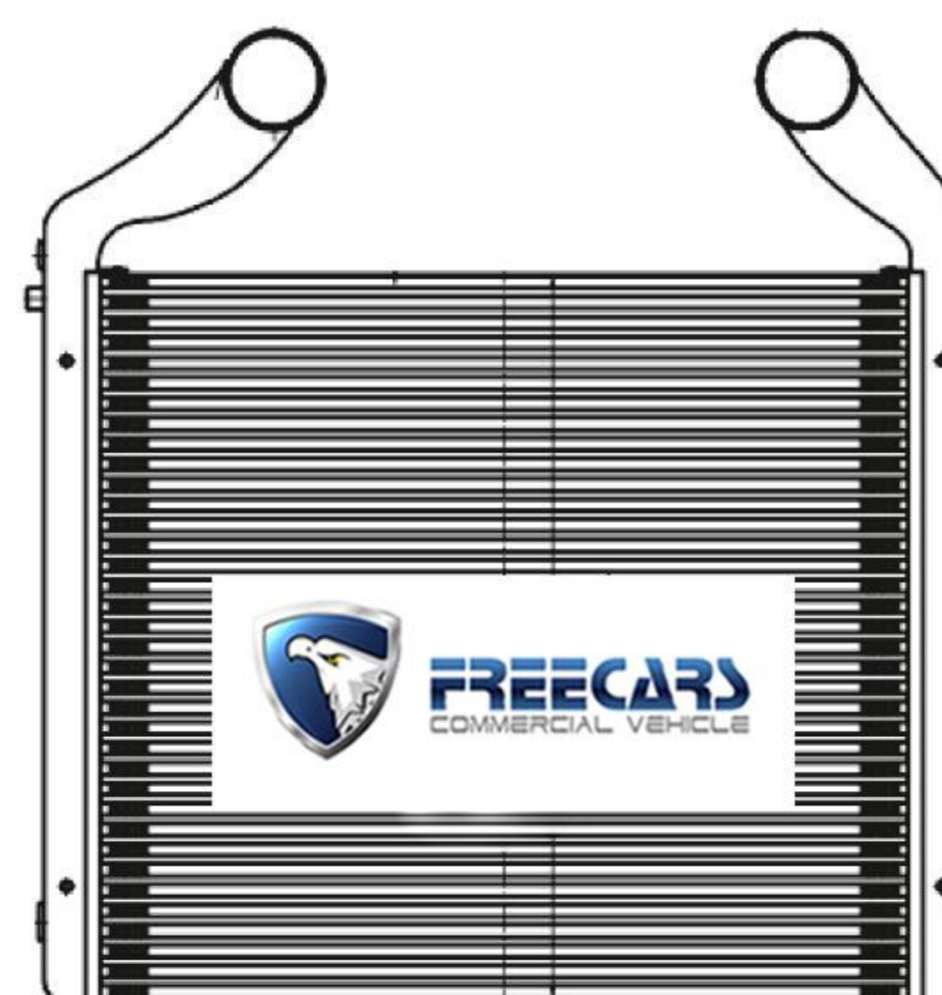
SACT-06 CORE SIZE:868*715*50 APP: SINOTRUK OEM:712W06100-0103
