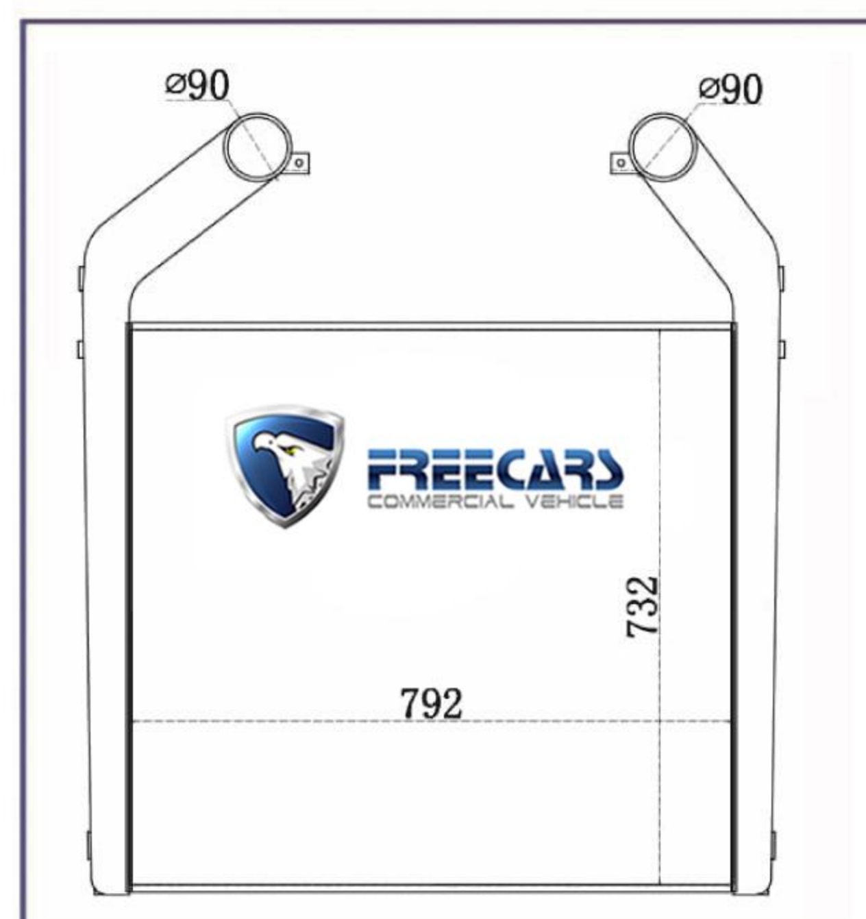
SACT-10 CORE SIZE:792*732*50 APP: SINOTRUK OEM:YZ9725530000899
