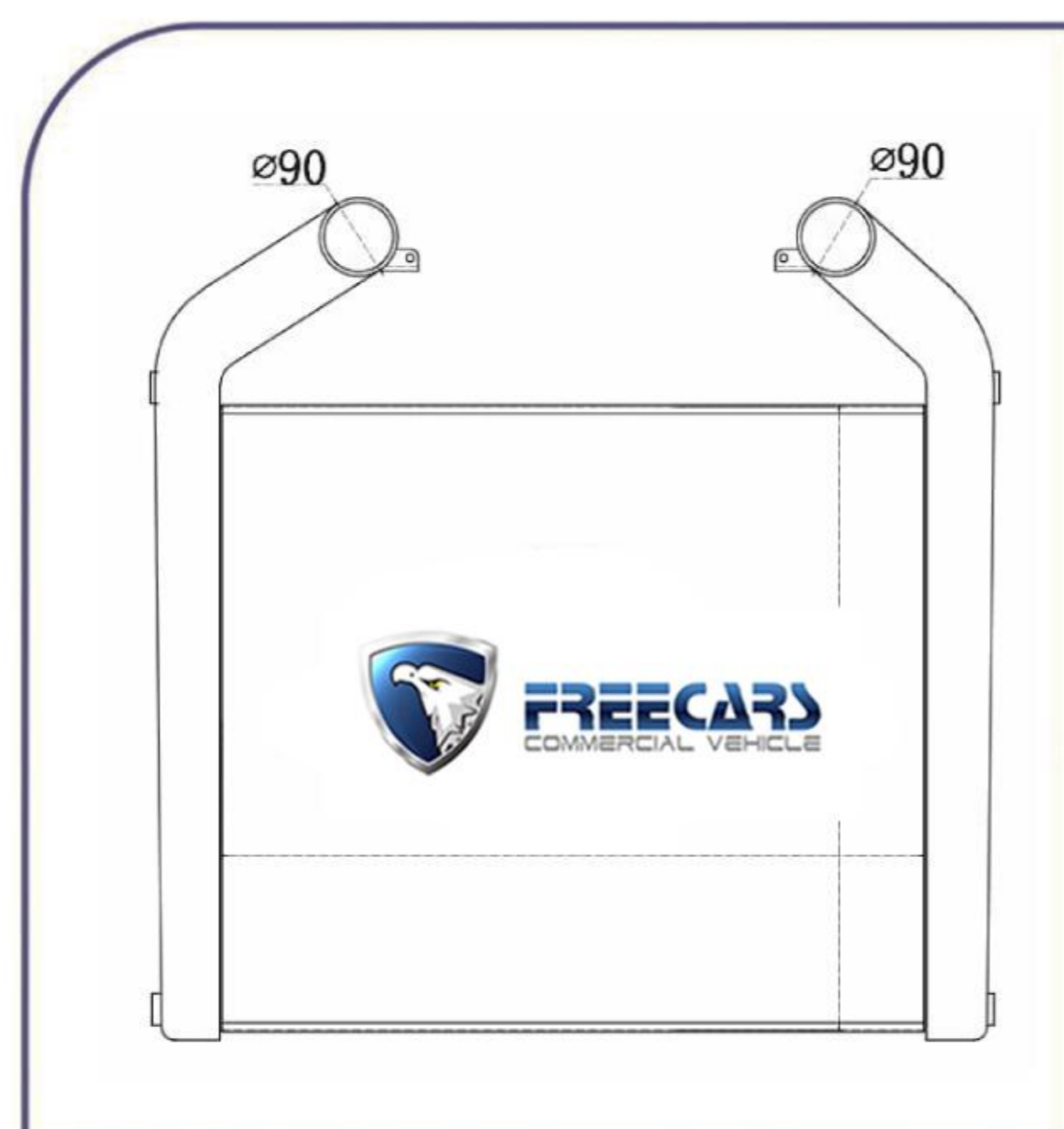
SACT-07 CORE SIZE:800*712*50 APP: SINOTRUK OEM:AZ962553000017-1
