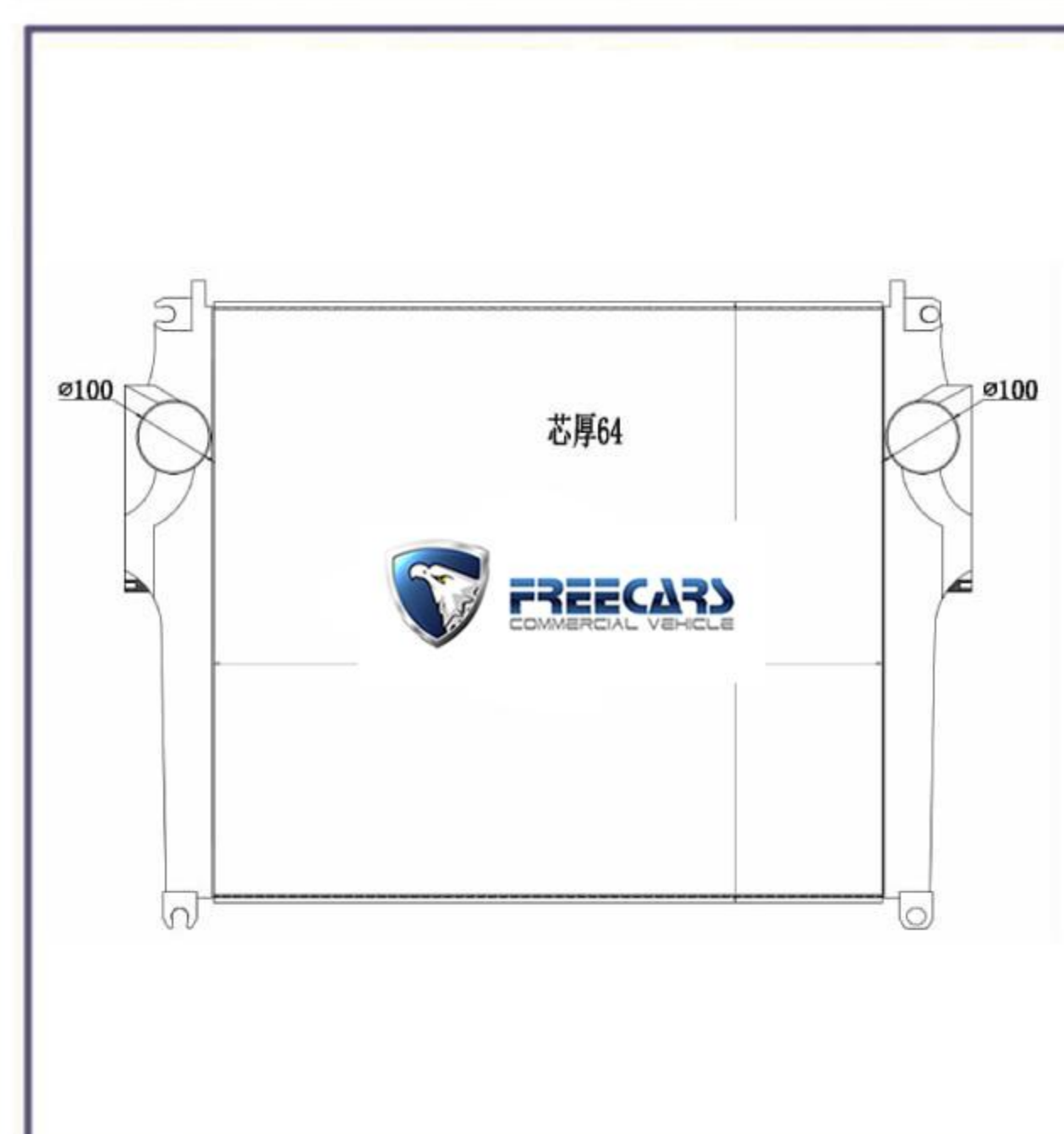
SACT-12 CORE SIZE:895*812*64 APP: SHACMAN OEM:DZ9X259531004
