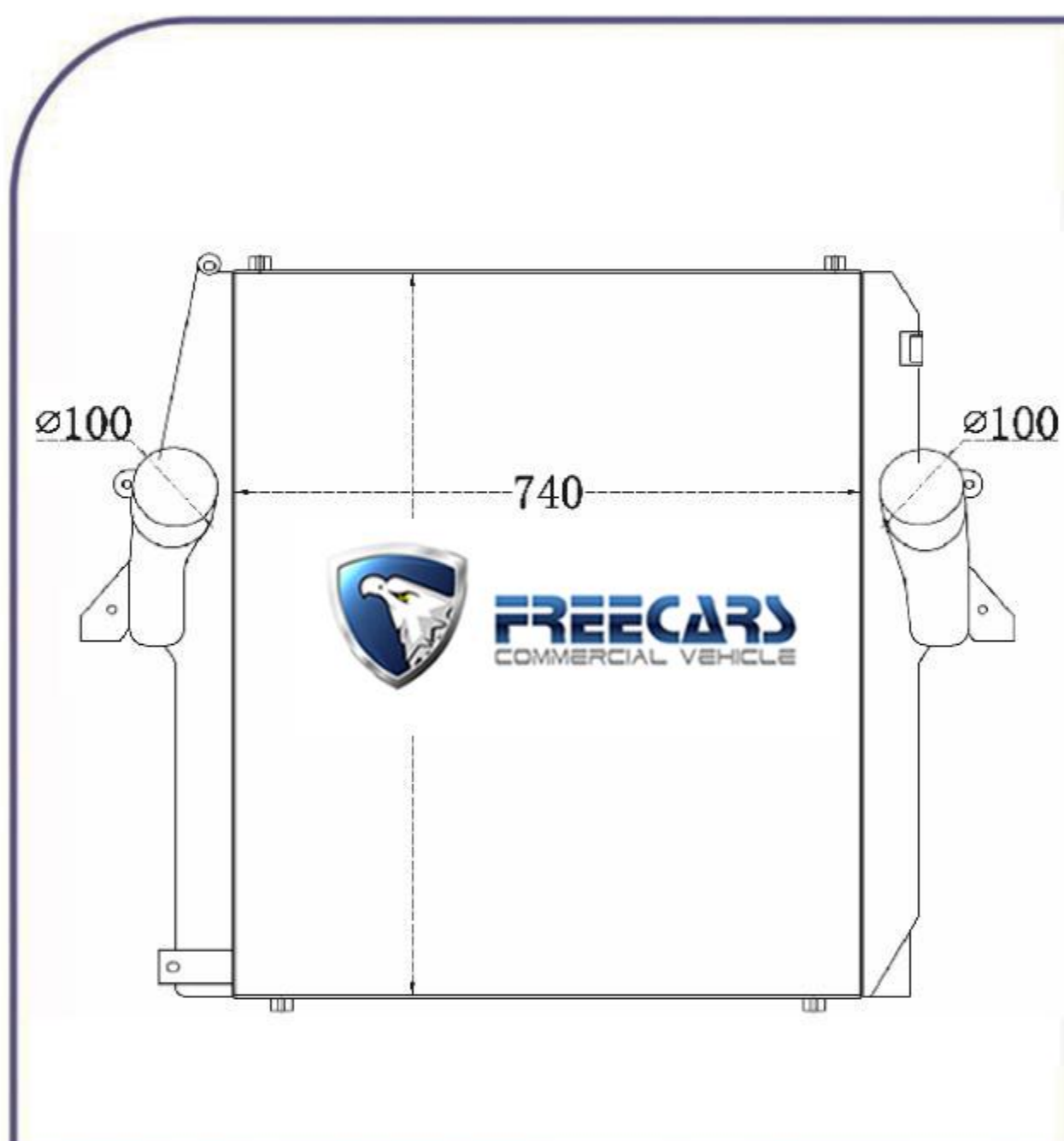
SACT-19 CORE SIZE:740*852*62 APP: XCMG OEM:NXG1119WLFW6B1 -010
