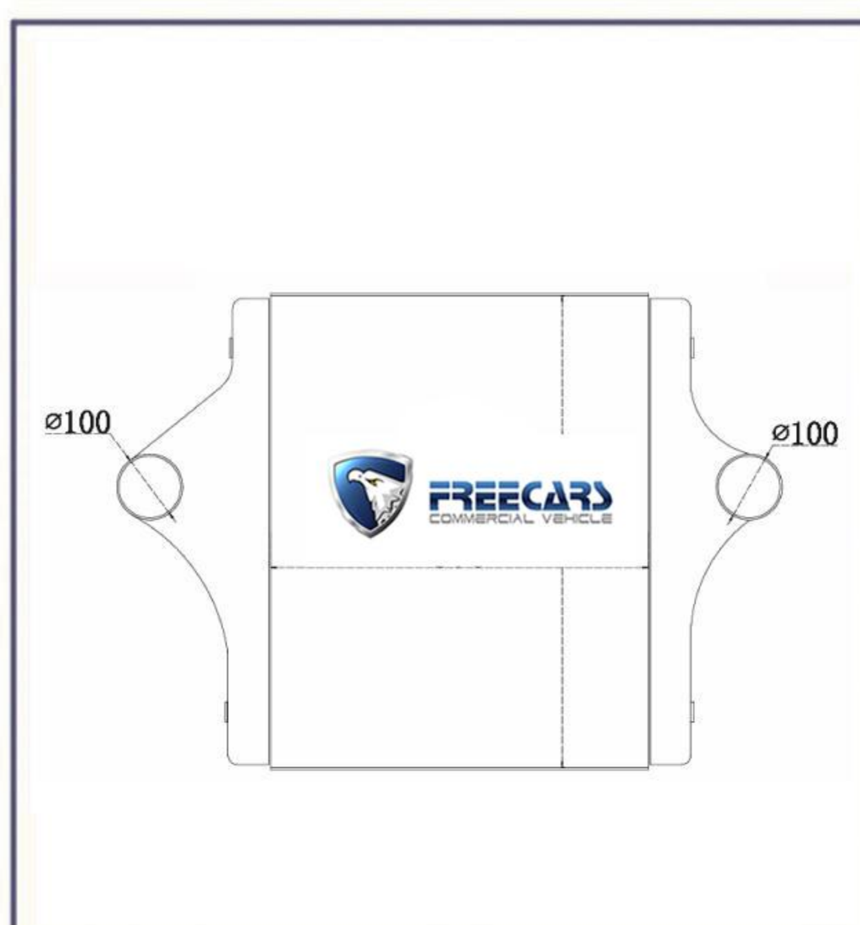
SACT-11 CORE SIZE:570*712*62 APP: SHACMAN OEM:DZ96259531030
