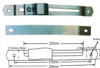
FCS-MUDG-016 MUDGUARD BRACKET OEM:
