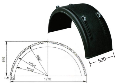
FCS-MUDG-018 UNIVERSAL MUDGUARD (WITH RUBBER LAYER) OEM:
