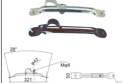
FCS-MUDG-045 MUDGUARD BRACKET OEM:
