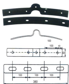
FCS-MUDG-013 MUDGUARD DECORATIVE BOARD OEM:
