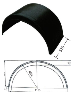
FCS-MUDG-010 MUDGUARD COVER OEM:
