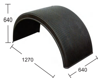
FCS-MUDG-021 UNIVERSAL MUDGUARD (WAVY) OEM:
