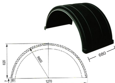
FCS-MUDG-023 UNIVERSAL MUDGUARD (WITH WHITE GARNISH) OEM:
