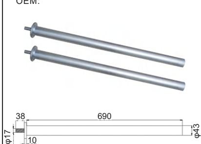
FCS-MUDG-046 MUDGUARD BRACKET OEM:
