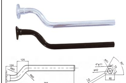
FCS-MUDG-043 MUDGUARD BRACKET OEM:
