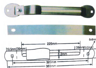
FCS-MUDG-015 MUDGUARD BRACKET OEM:
