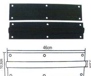
FCS-MUDG-014 MUDGUARD DECORATIVE BOARD OEM:
