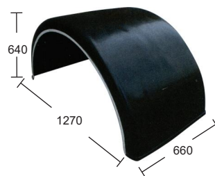
FCS-MUDG-026 MUDGUARD OEM:
