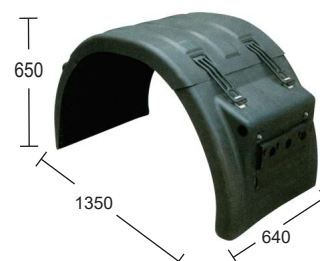
FCS-MUDG-020 UNIVERSAL MUDGUARD OEM:
