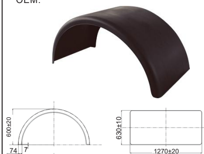
FCS-MUDG-035 MUDGUARD OEM:
